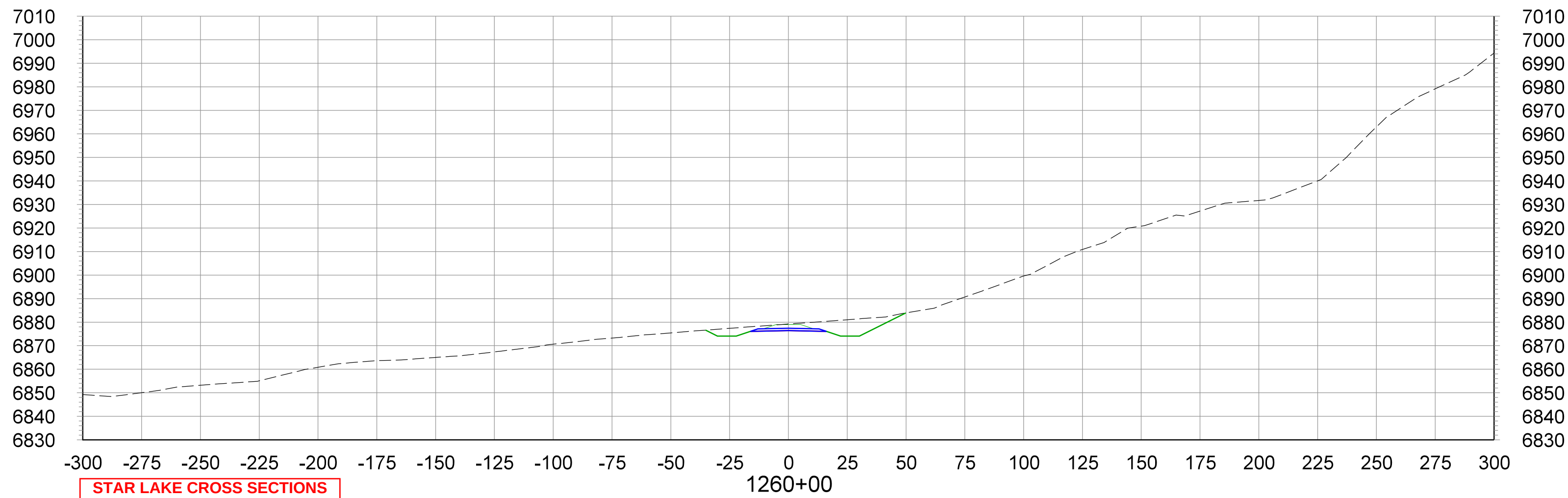
CROSS SECTIONS STA.1260+00 TO STA.1265+00
