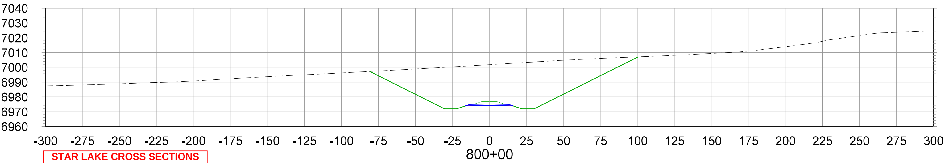
CROSS SECTIONS STA.800+00 TO STA.815+00
