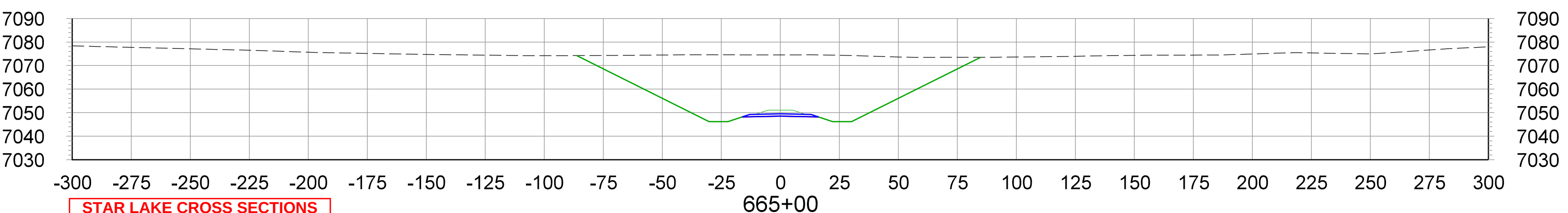
CROSS SECTIONS STA.665+00 TO STA.680+00
