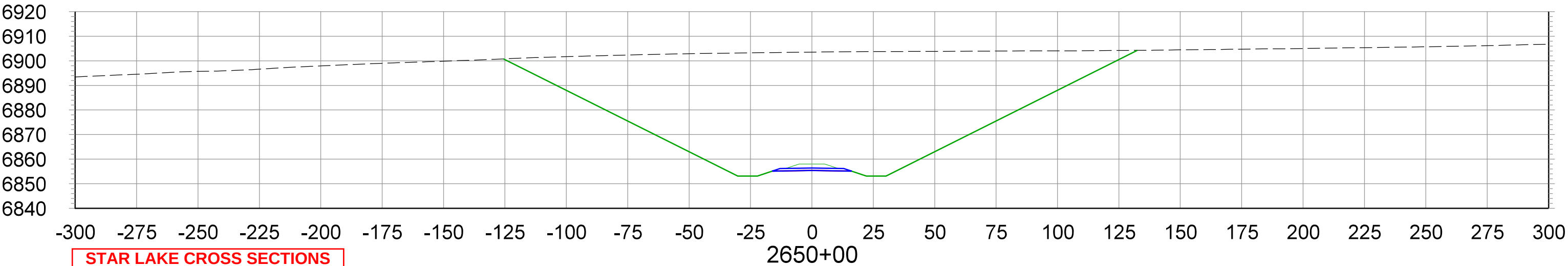
CROSS SECTIONS STA.2650+00 TO STA.2660+00
