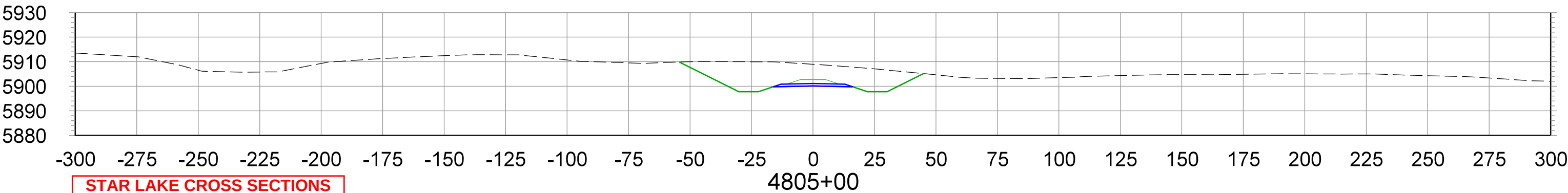
CROSS SECTIONS STA.4805+00 TO STA.4820+00
