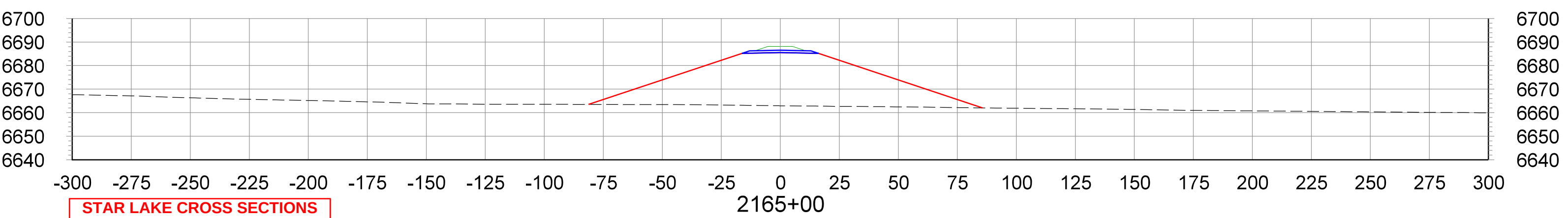
CROSS SECTIONS STA.2165+00 TO STA.2180+00
