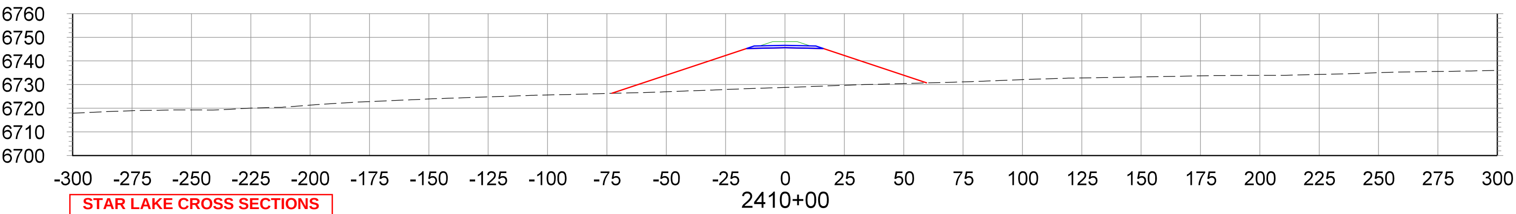
CROSS SECTIONS STA.2410+00 TO STA.2425+00
