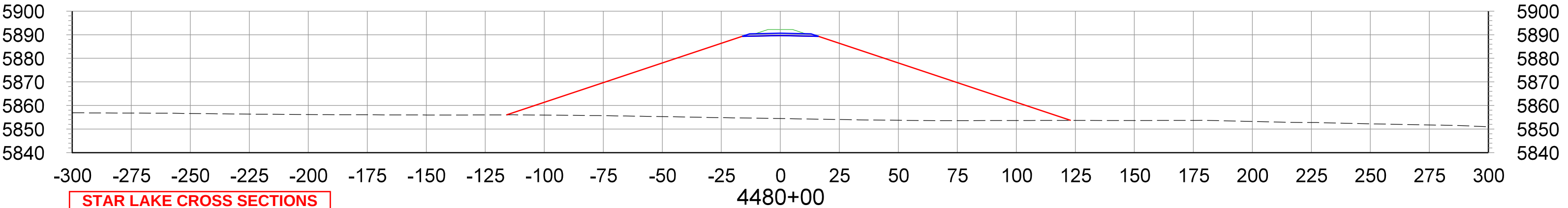
CROSS SECTIONS STA.4480+00 TO STA.4495+00
