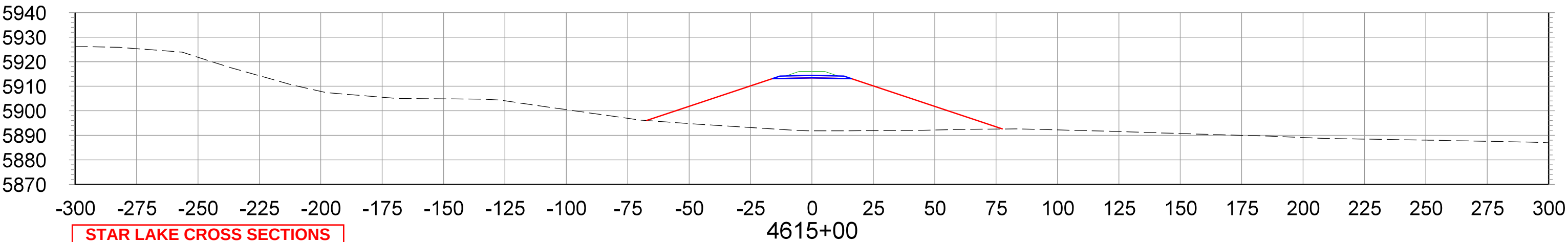
CROSS SECTIONS STA.4615+00 TO STA.4630+00
