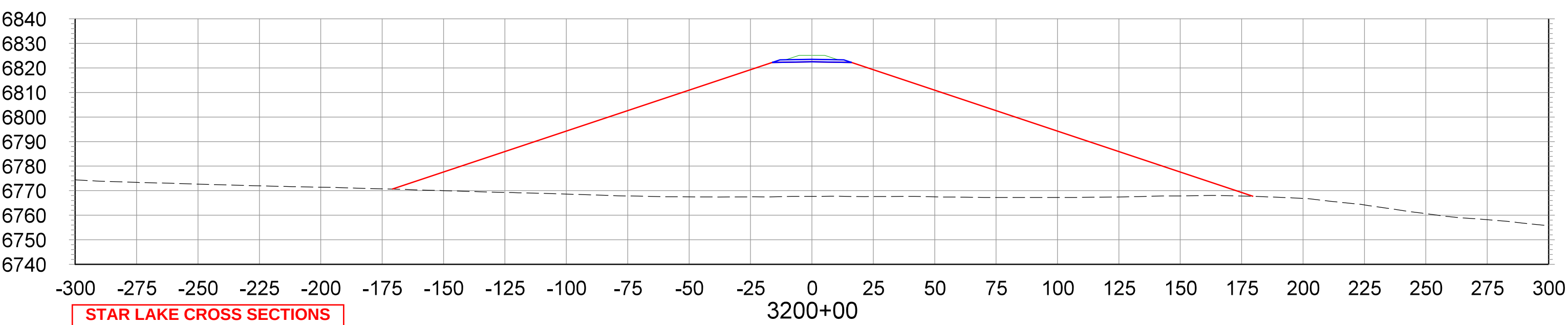
CROSS SECTIONS STA.3200+00 TO STA.3210+00
