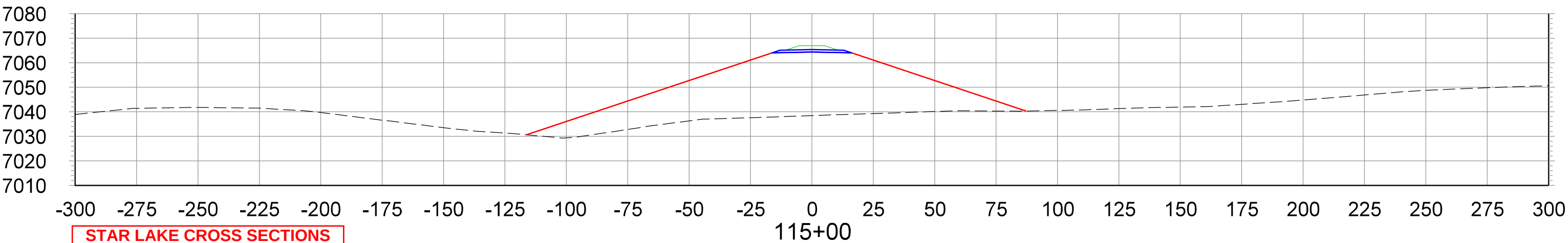
CROSS SECTIONS STA.115+00 TO STA.130+00
