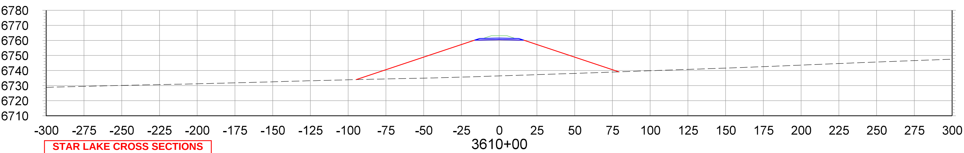
CROSS SECTIONS STA.3610+00 TO STA.3625+00
