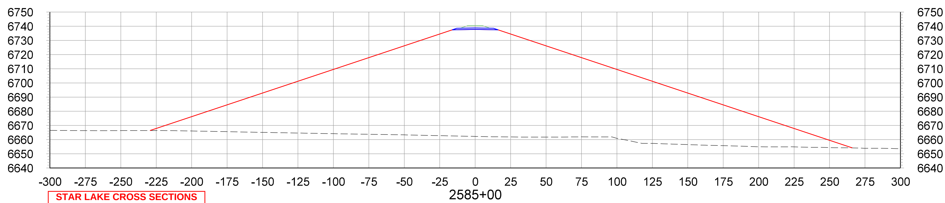
CROSS SECTIONS STA.2585+00 TO STA.2590+00
