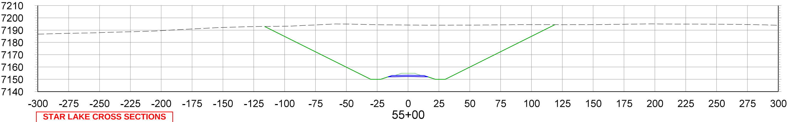
CROSS SECTIONS STA.55+00 TO STA.70+00
