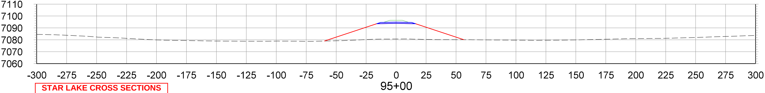
CROSS SECTIONS STA.95+00 TO STA.110+00
