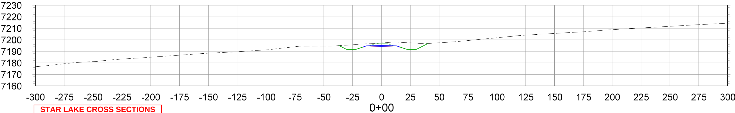
CROSS SECTIONS STA.0+00 TO STA.10+00
