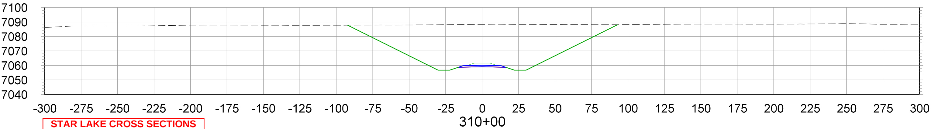
CROSS SECTIONS STA.310+00 TO STA.325+00
