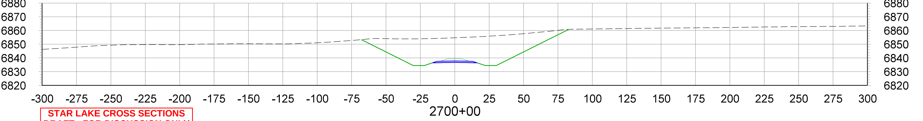
CROSS SECTIONS STA.2700+00 TO STA.2715+00
