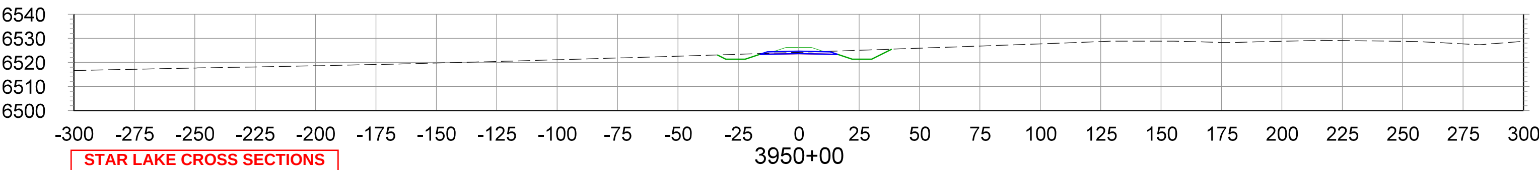
CROSS SECTIONS STA.3950+00 TO STA.3965+00
