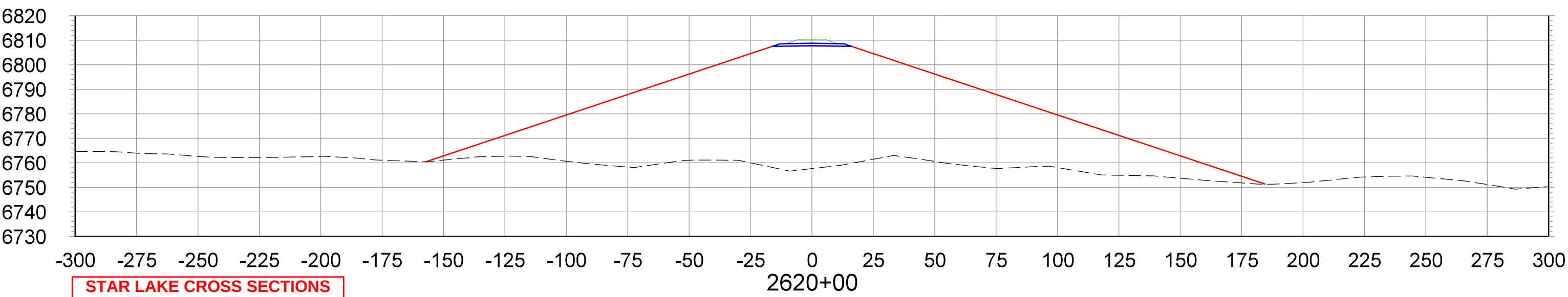
CROSS SECTIONS STA.2620+00 TO STA.2630+00
