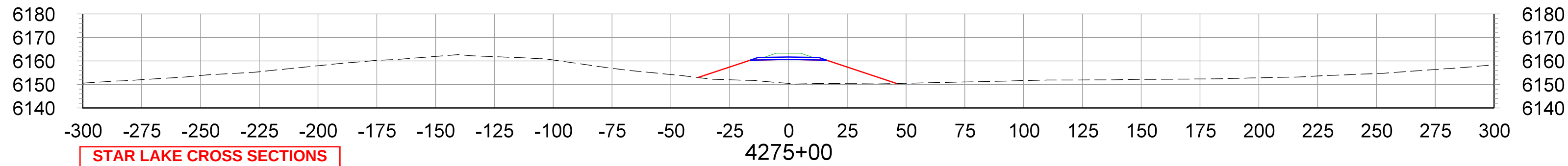
CROSS SECTIONS STA.4275+00 TO STA.4290+00
