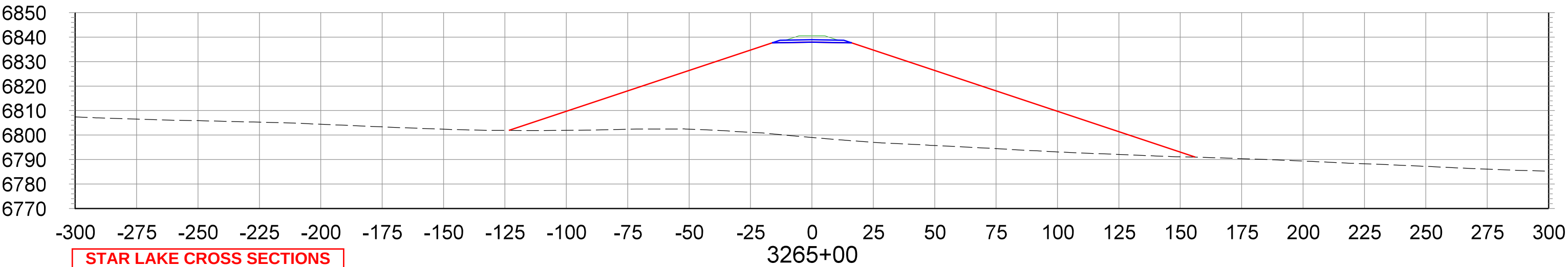
CROSS SECTIONS STA.3265+00 TO STA.3280+00
