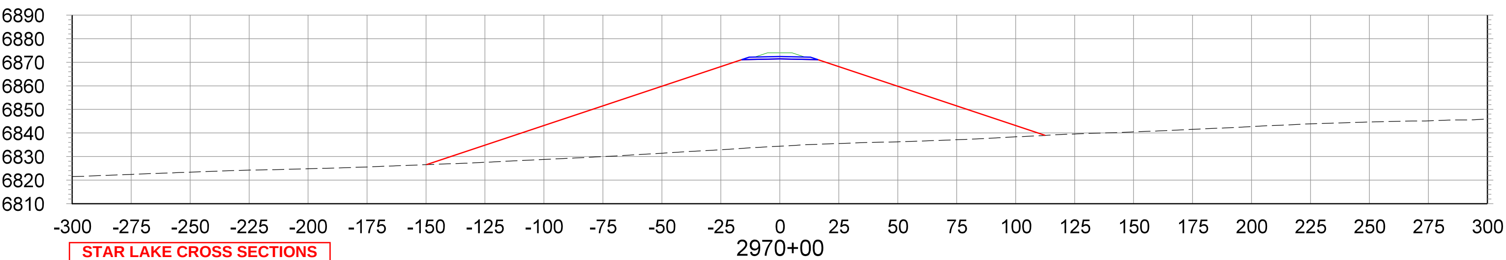
CROSS SECTIONS STA.2970+00 TO STA.2985+00
