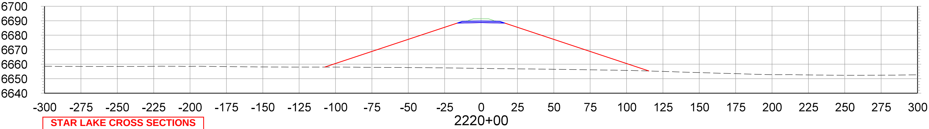
CROSS SECTIONS STA.2220+00 TO STA.2235+00
