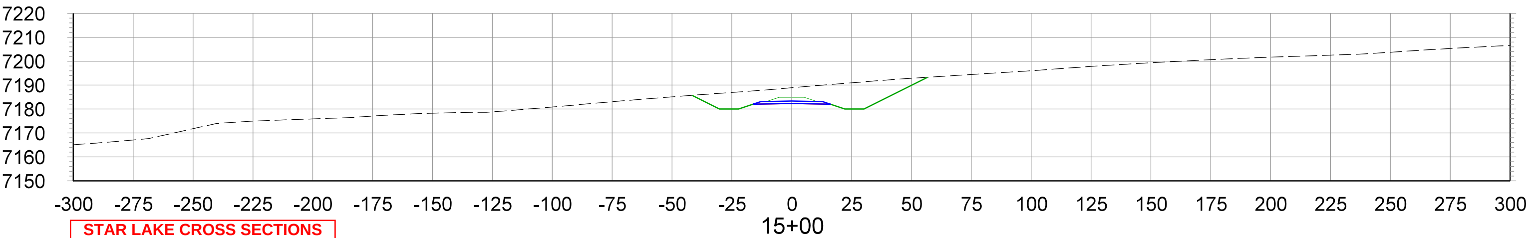
CROSS SECTIONS STA.15+00 TO STA.30+00
