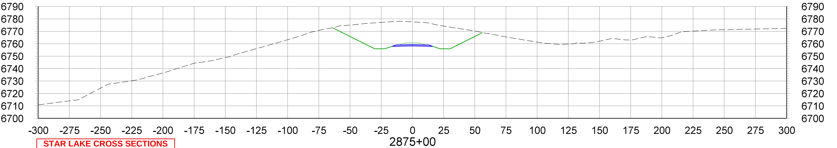
CROSS SECTIONS STA.2875+00 TO STA.2885+00
