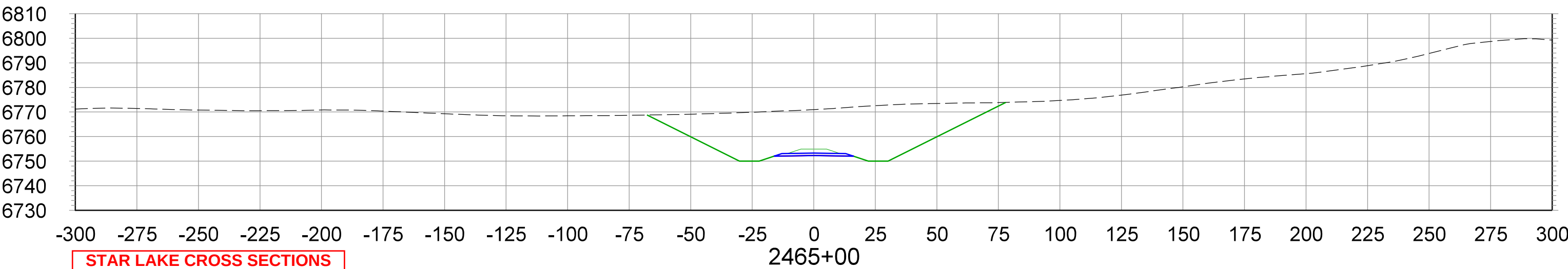
CROSS SECTIONS STA.2465+00 TO STA.2480+00
