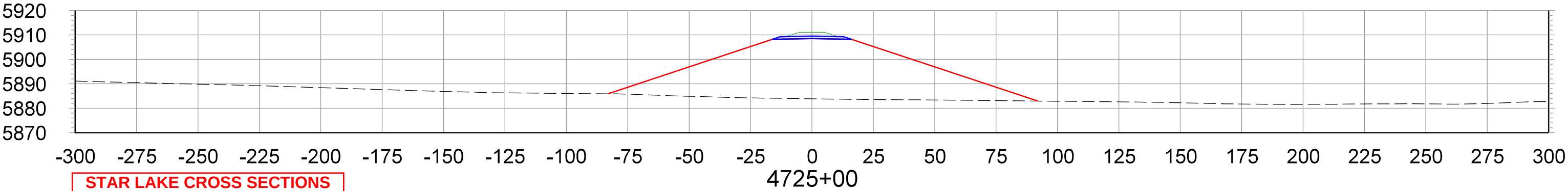
CROSS SECTIONS STA.4725+00 TO STA.4740+00
