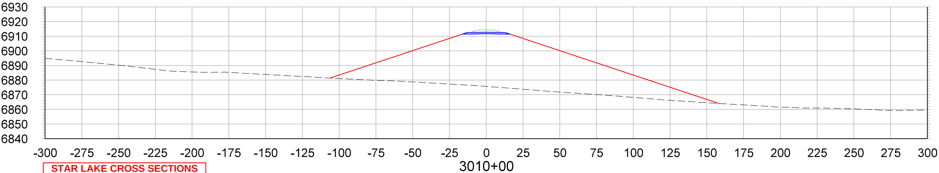
CROSS SECTIONS STA.3010+00 TO STA.3020+00
