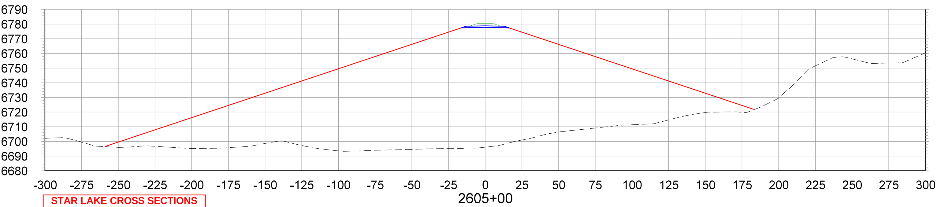
CROSS SECTIONS STA.2605+00 TO STA.2615+00
