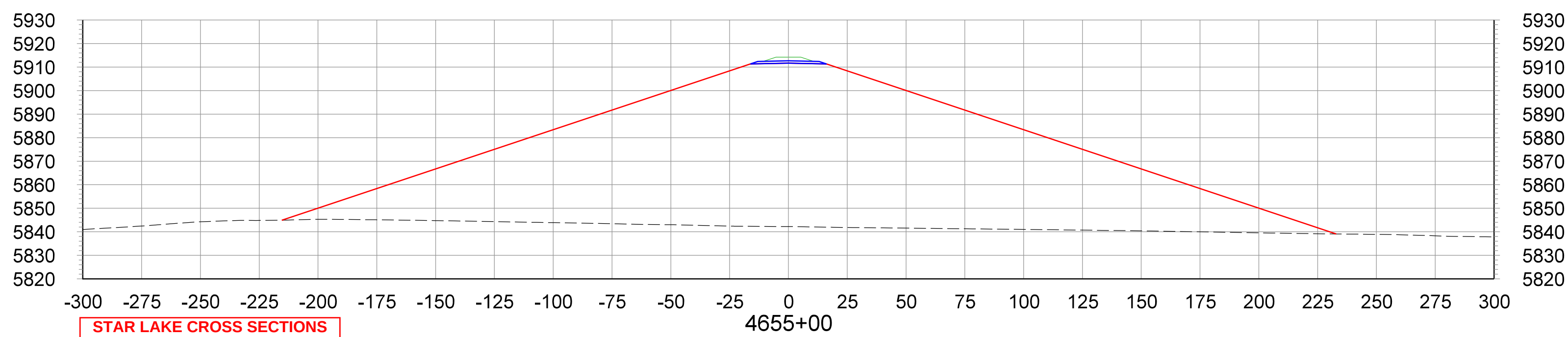
CROSS SECTIONS STA.4655+00 TO STA.4660+00
