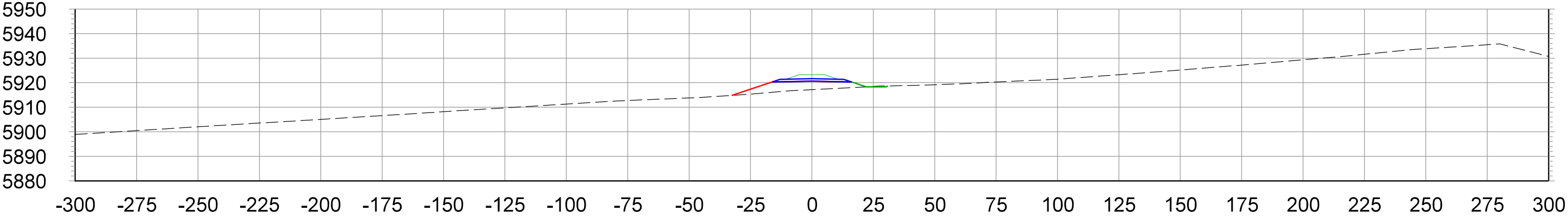
CROSS SECTIONS STA.4445+00 TO STA.4460+00
