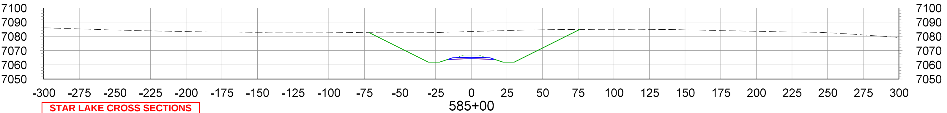
CROSS SECTIONS STA.585+00 TO STA.600+00
