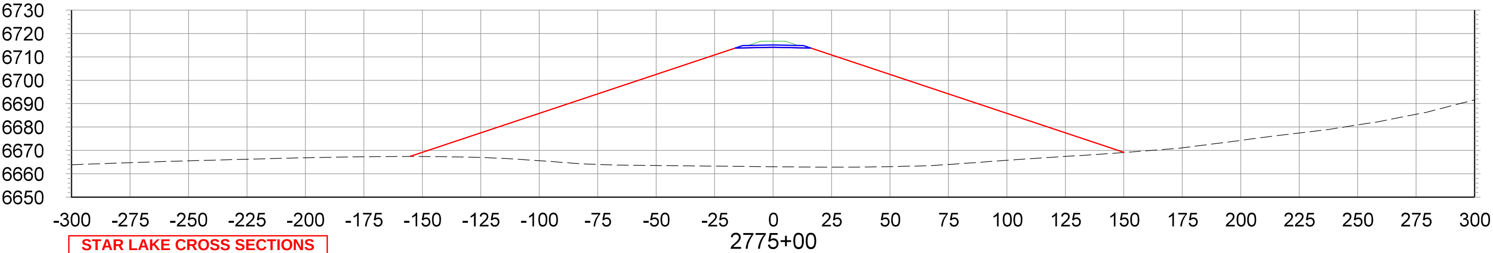
CROSS SECTIONS STA.2775+00 TO STA.2785+00
