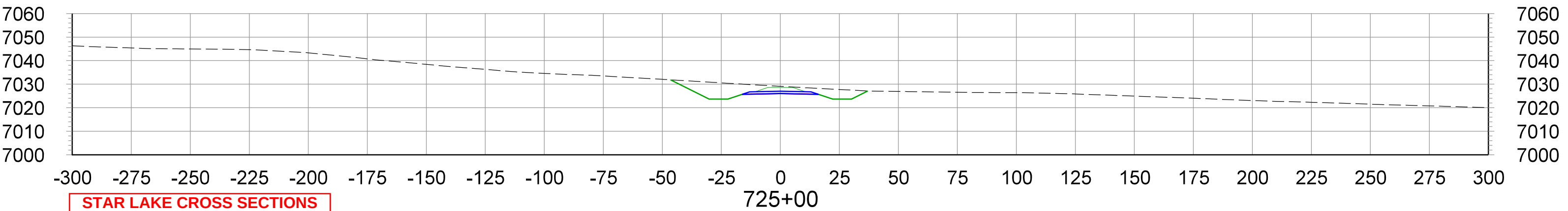
CROSS SECTIONS STA.725+00 TO STA.740+00
