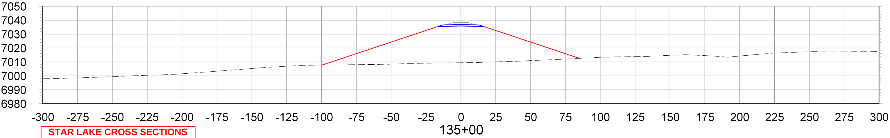
CROSS SECTIONS STA.135+00 TO STA.150+00
