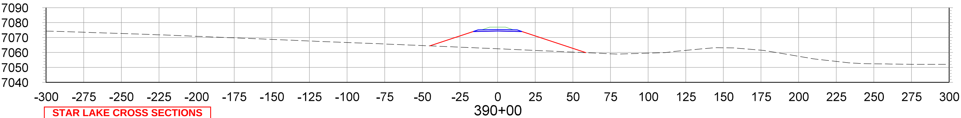
CROSS SECTIONS STA.390+00 TO STA.405+00
